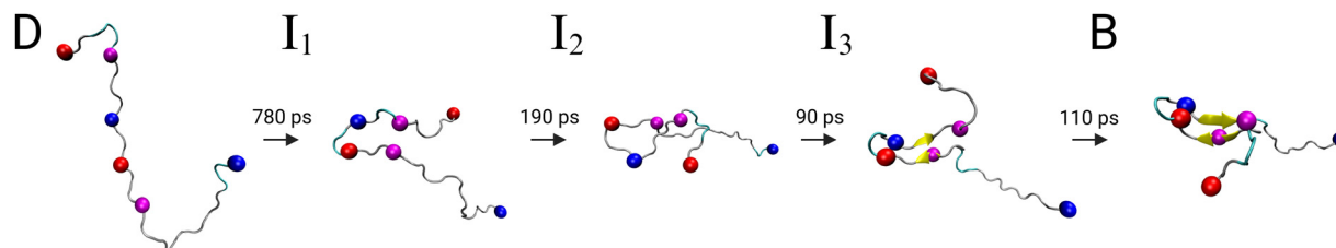
Fig. 3 Fastest pathway from the intrinsically disordered state (D) to the global minimum (B) in the dimer free energy surface. The spheres represent the centroids used in the DRID metric. The FPTs associated with the fastest transition between the states along the pathway are shown above the arrows, which were calculated separately for each transition and therefore do not add up to the total transition time associated with the full pathway, where all possible recrossing events are included. Fig. S1 (ESI ^\dagger ) shows the pathway again, but with both peptides within the dimer.
